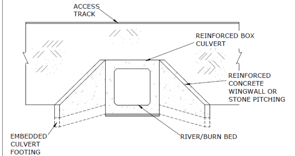
TYPICAL BOX CULVERT ELEVATION (NTS)
